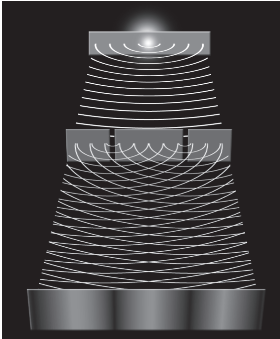
Figure 3: Electron Bombardment of Double Slits
