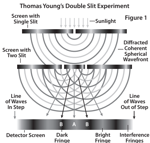
Figure 2: Thomas Young's Famous Double Slit Experiment
